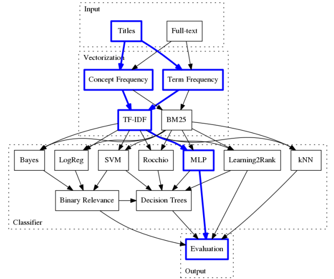
Figure 1: Configurable text-processing pipeline used for our experiments. The best-performing strategy is emphasized.
