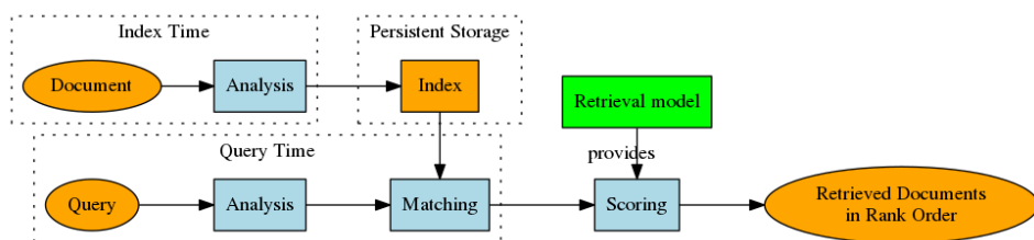
Fig. 1: A simplified information retrieval system.
