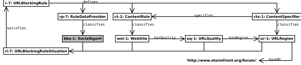
(a) First example flow control rule of the Application-Level Proxy Ontology
