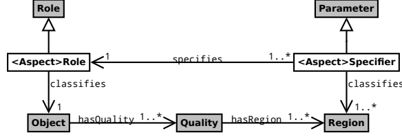
Fig. 3. Basic structure of a communication aspect in the Flow Control Rule Pattern. <Aspect> is a placeholder for Sender, Receiver, Content, and Channel.
