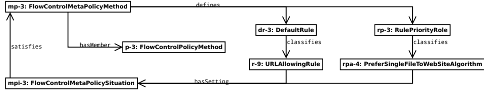
(d) Example flow control meta-policy of the Application-Level Proxy Ontology
