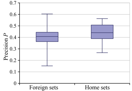
Figure 12. Results for S_{b+e} for foreign and home sets.
