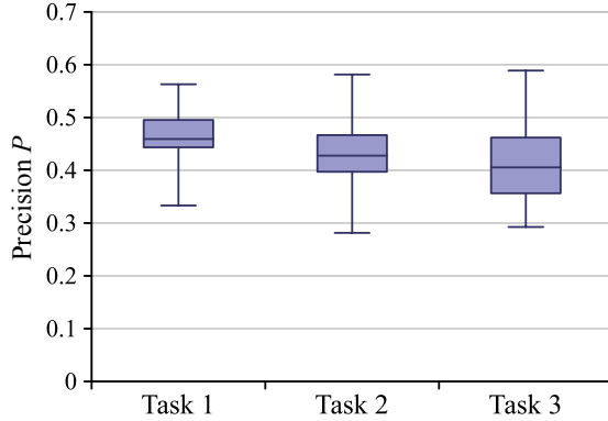
Figure 13. Results for S_{b+e} for different selection tasks.
