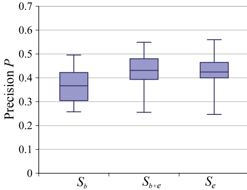
Figure 10. Precision results for all users averaged over 30 random splits obtained from combining measures by logistic regression. The results are based on baseline measures S_b , eye tracking measures S_e , and all measures S_{b+e} .
