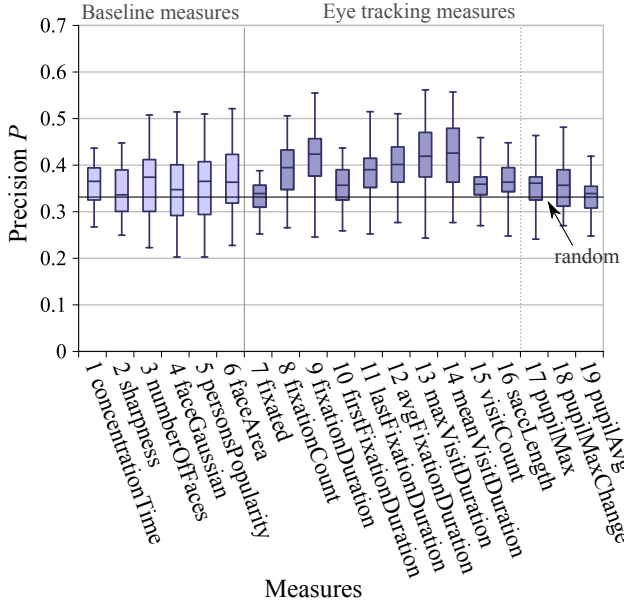
Figure 9. Precision results for all users averaged over 30 random test sets when selecting the photos based on single measures.
