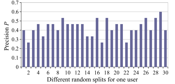
Figure 11. Precision results for S_{b+e} over 30 different random splits for one user.
