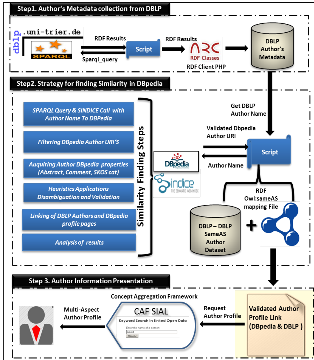
Figure 1. Similarity Finding Framework
