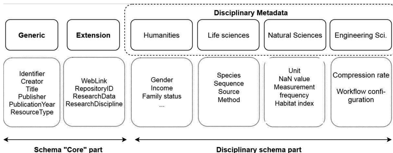
Fig. 1: GeRDI Schema components
